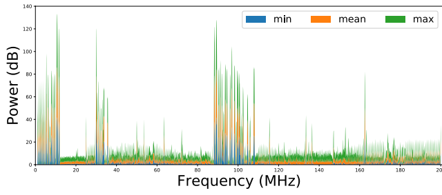
Figure 8. RF power density from 1 to 200MHz.
