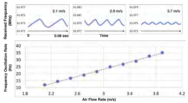
Figure 16. Top: received Sozu tag frequency at different wind speeds. Bottom: the linear correlation between Sozu-detected frequency oscillation rate and actual wind speed.
