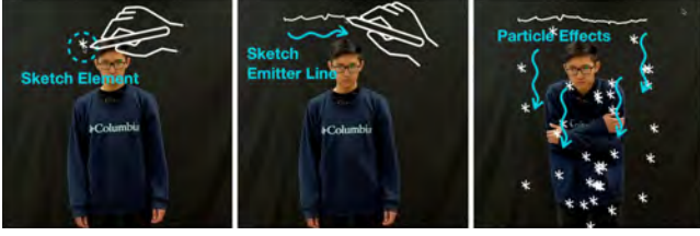
Figure 8: Particle Effects
