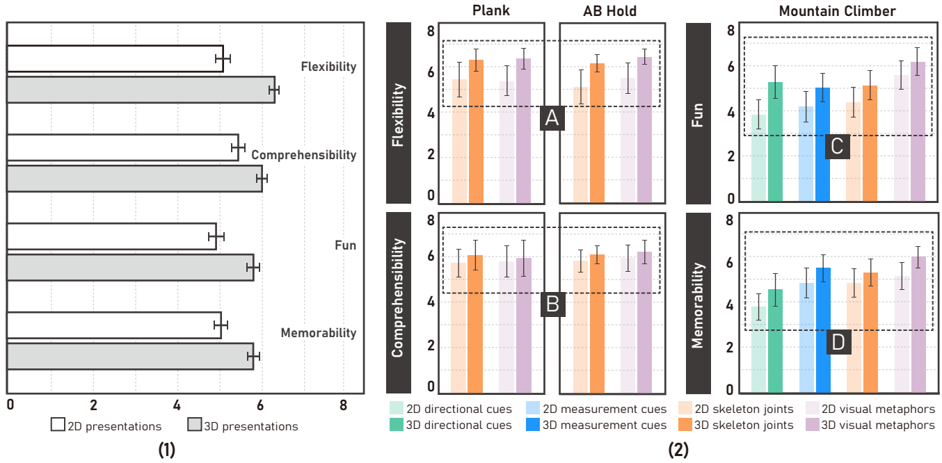
Figure 11: (1) User ratings for all the 2D/3D presentations. (2) Typical user ratings from several workouts, where each color indicates the type of visual cue, and transparency is used to distinguish 2D/3D. Error bars denote 95% confidence intervals, and the complete figure is available in the supplementary material.
