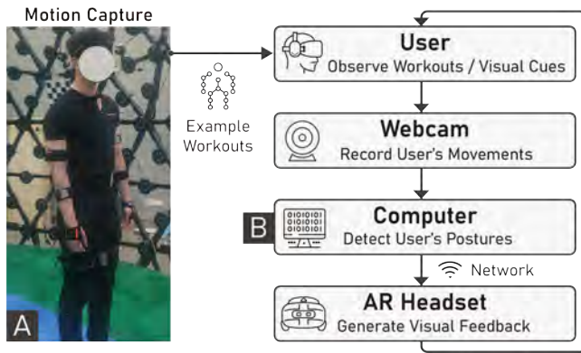
Figure 7: The workflow of AR-based physical training.
