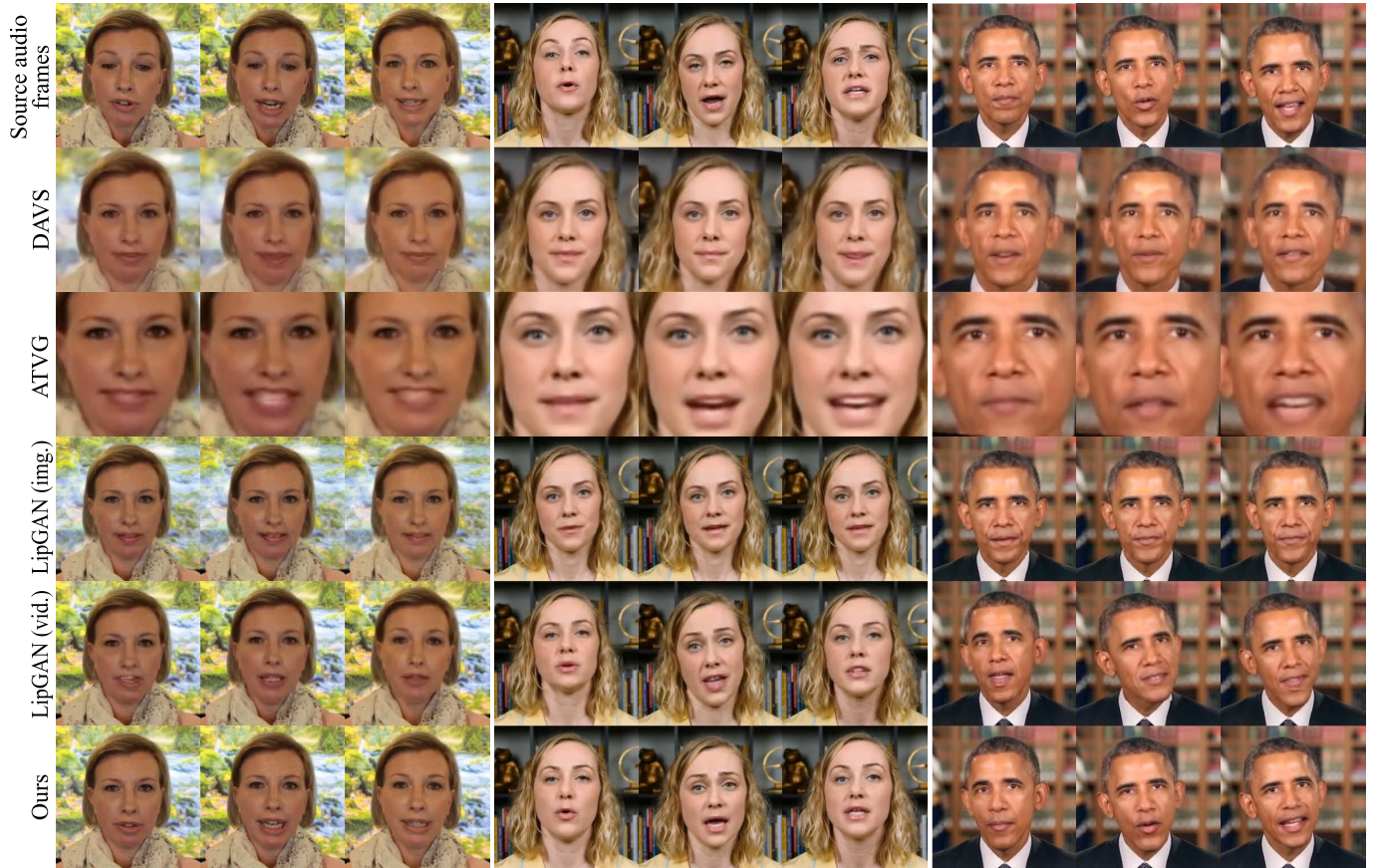
Fig. 10. Comparison to DAVS [63], ATVG [11] and LipGAN [40] on target videos A , B and I . Top: sampled video frames corresponding to the source audio tracks. Second row to the bottom: corresponding video portrait frames from different methods. Our approach generates more natural-looking results with precise mouth synchronization to the audio, higher quality mouth interior and better temporal stability.
