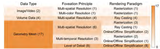
Fig. 6 Frequency of research in foveated rendering from 1990 to 2011. Numbers in parentheses indicate the number of studies using the specific data type, foveated principle and rendering paradigm are listed in front of parentheses.
