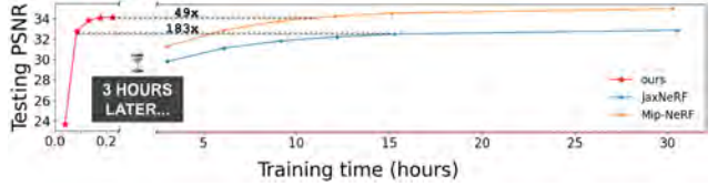
(b) The training curves of different methods on Lego scene. The training time of each method is measured on our machine with a single NVIDIA RTX 2080 Ti GPU.
