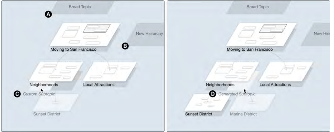
Figure 4: Hierarchy view: Users can add (A) a canvas above (e.g., ‘Relocating to a new city’ above ‘Moving to San Francisco’) or (B) another hierarchy on the side (e.g., ‘Moving to San Jose’ next to ‘Moving to San Francisco’). To add a subtopic canvas, users can click (c) Custom Subtopic and specify the topic (e.g., ‘Sunset District’) or (D) Generated Subtopic to have LLM suggest a subtopic (e.g., ‘Marina District’).
