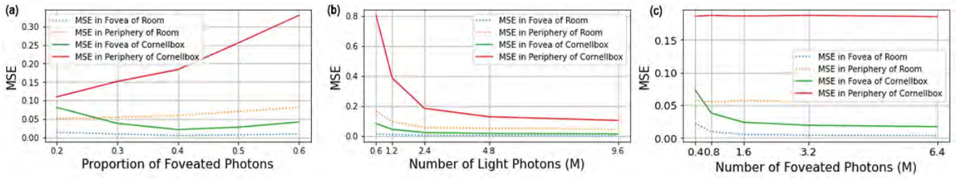
Fig. 6: MSE in Room and Cornellbox as a function of (a) the proportion of foveated photons in total photons \frac{N_f}{N_l+N_f} , (b) the number of light photons N_l , and (c) the number of foveated photons N_f .
