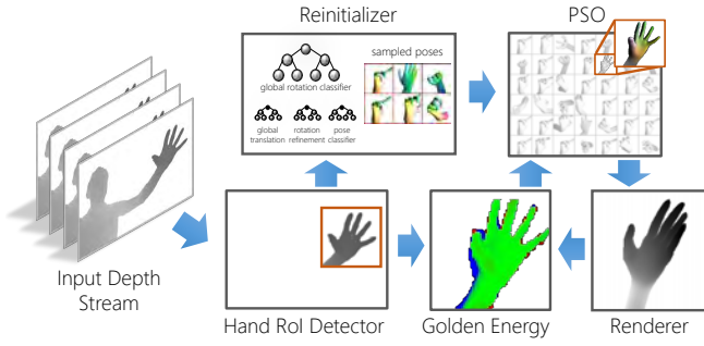
Figure 2: Algorithm pipeline.
