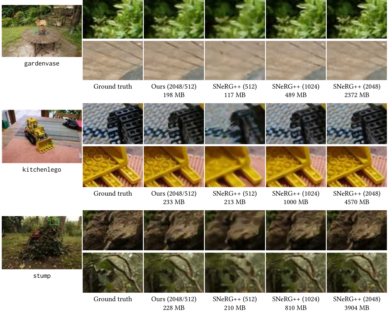
Fig. 5. Visual comparison between MERF and various resolution SNeRG++ [Hedman et al. 2021] models. Total VRAM (GPU memory) usage during rendering is listed beneath each method name. Only SNeRG++ (512) has comparable size to our model, whereas SNeRG++ (1024) and SNeRG++ (2048) are significantly larger.
