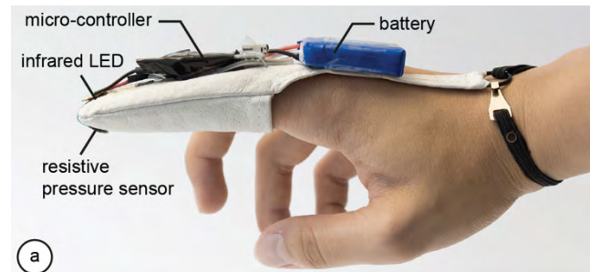
Figure 5: Tracking unit.
