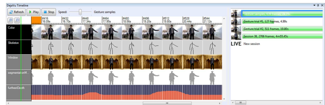
Figure 6: DejaVu Timeline.
