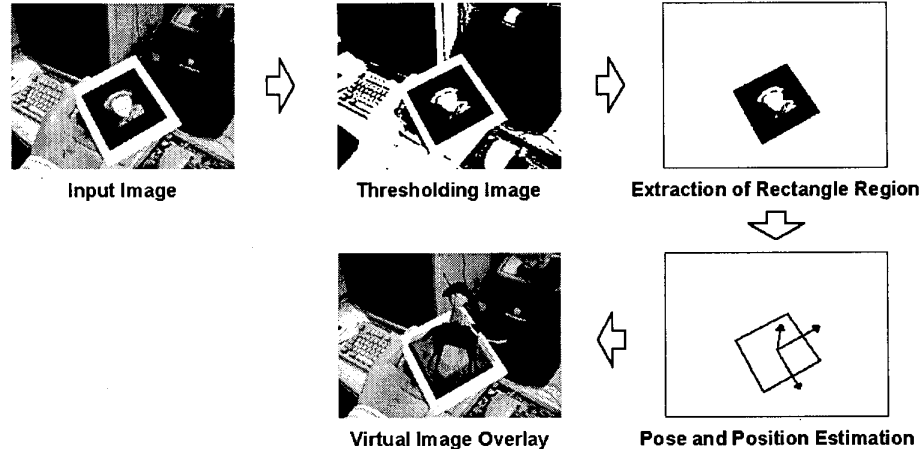
Figure 4: The Vision-Based AR Tracking Process
