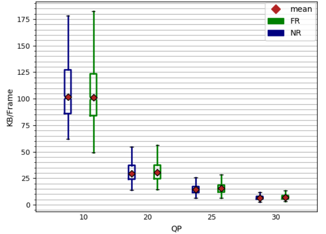
Figure 8: Comparison of frame sizes with foveated rendering (FR) and normal rendering (NR) with different QP values.
