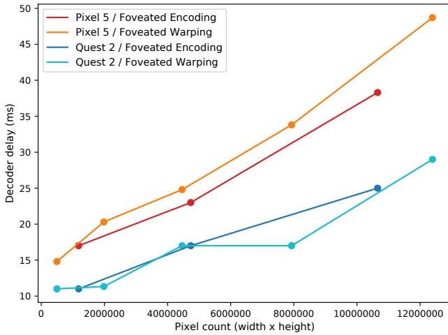
Figure 12: Decoder delay when increasing pixel count using Foveated Encoding or Foveated Warping.
