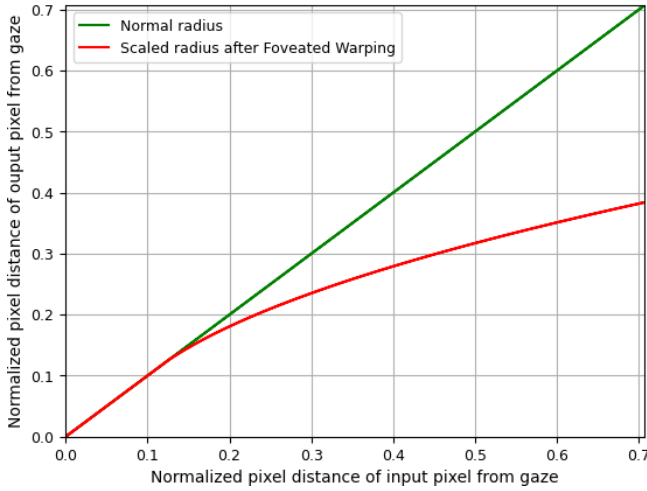
Figure 6: The distance of pixel from gaze fixation point changes with foveated warping (red curve).
