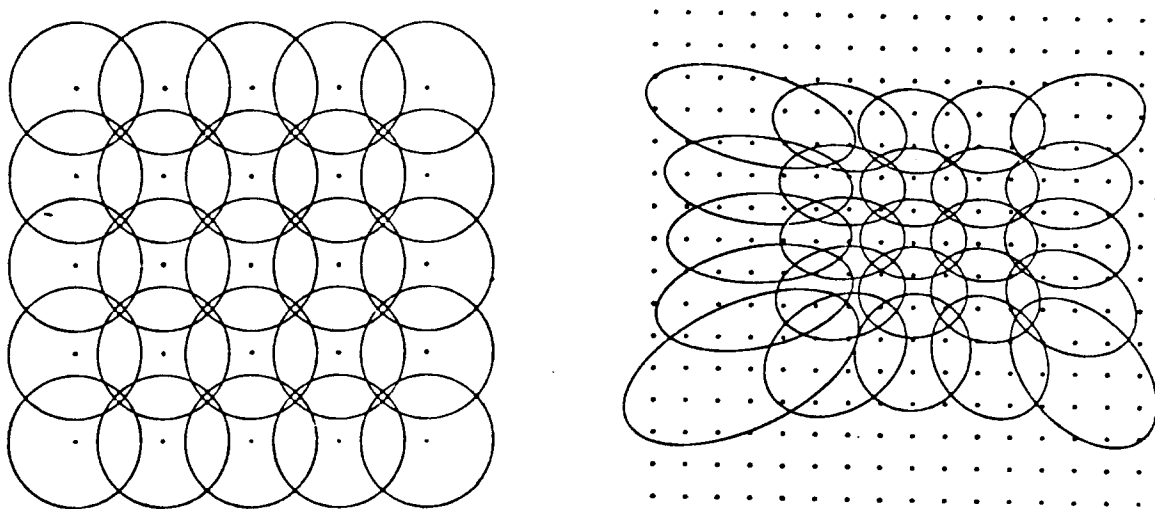
Figure 3.15: A nonuniform resampling grid and the corresponding space variant filter regions. Circular regions in screen space (left) map to elliptical regions in texture space (right). Since the texture regions vary in size, eccentricity, and orientation, the filter is space variant. Dots mark pixel centers.
