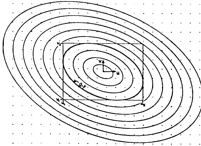
Figure 3.20: Regions of an elliptical Gaussian (or EWA) filter are concentric ellipses. Dots are texture pixel centers. Algorithm scans pixels inside box; only those inside the contour Q = F contribute to the weighted average.
