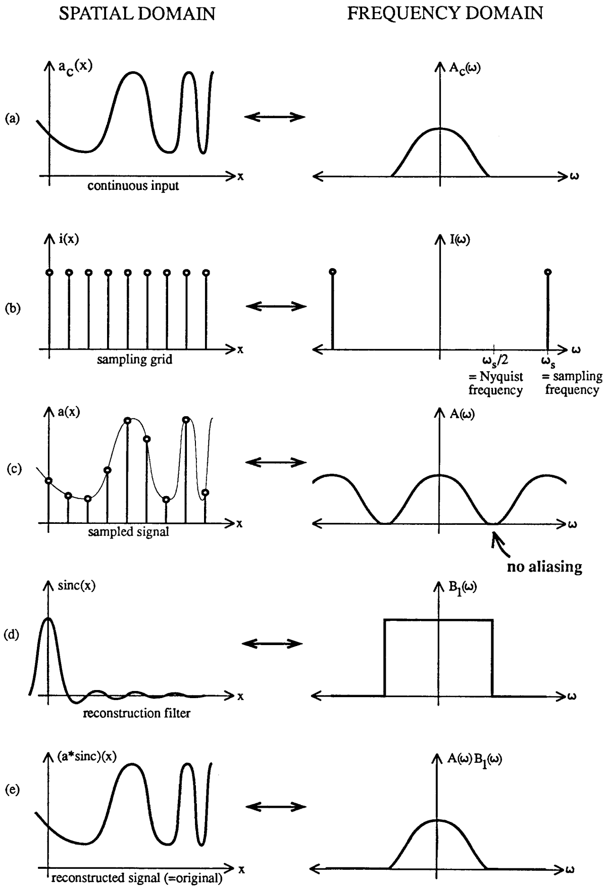
Figure 3.4: Sampling above the Nyquist rate (no aliasing).
