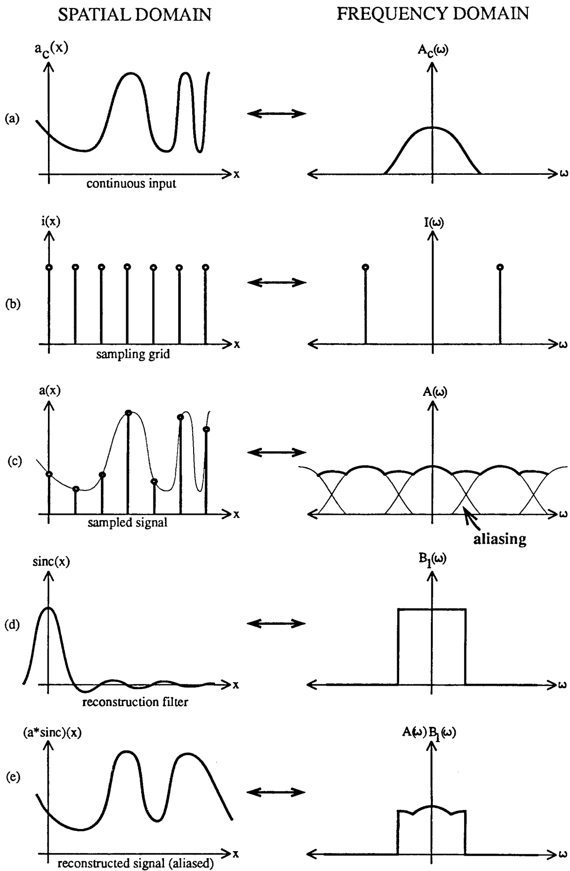
Figure 3.5: Sampling below the Nyquist rate (aliasing).
