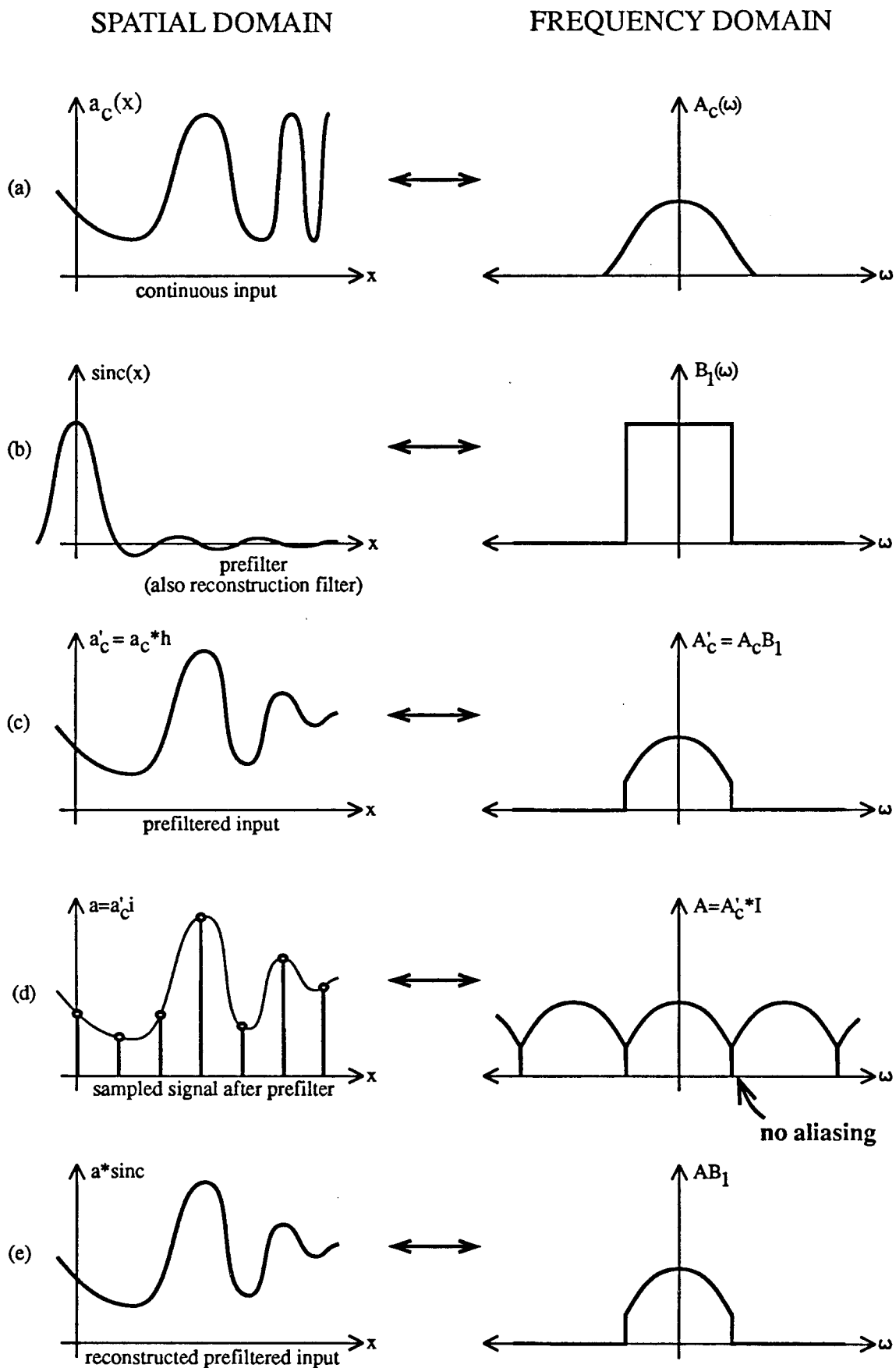
Figure 3.7: Ideal prefiltering eliminates aliasing.
