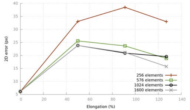
Figure 4: Registration error with respect to object elongation with a variation of mesh resolution: With an adequate number of tetrahedral elements the projection error can be significantly reduced.
