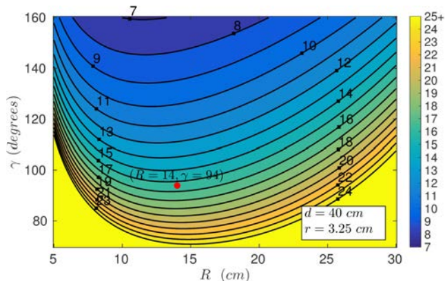
Figure 10: Minimum number of cameras as a function of rig radius R and horizontal field of view \gamma . The interpupillary distance is set to 6.5cm and the minimum distance d is set to 40cm. Increasing the number of cameras reduces field of view requirements while increasing the viewing circle radius increases the required field of view. The design choice in this work is shown as a large red dot at R = 14\text{cm} and \gamma = 94^\circ .
