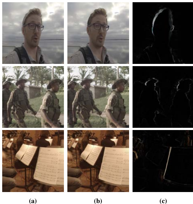
Figure 15: Compositing Methods. (a) Results by averaging all contributions to each pixel. (b) Results using our continuous compositing method. (c) The difference between (a) and (b).
