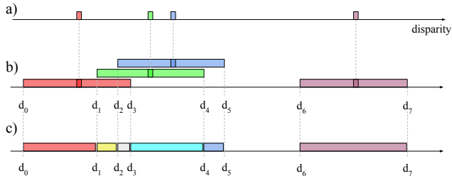
Figure 16: The stages of our interval-based compositing algorithm explained using a single pixel. (a) First, the splatting algorithm has assigned four fragments into the pixel. (b) Next, the fragments are expanded by applying a constant offset to both directions in disparity space. (c) Finally, spans of constant color are created and composited using the over-operator.
